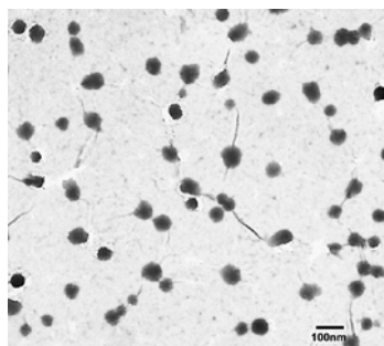
Figure 2. TEM image of nanoMIPs specific for melamine.
