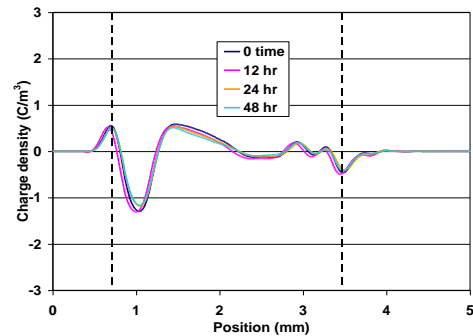
(a) Charge decay after positive voltage stressing
