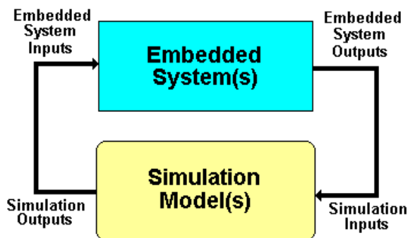
Fig. 9: HIL principle
