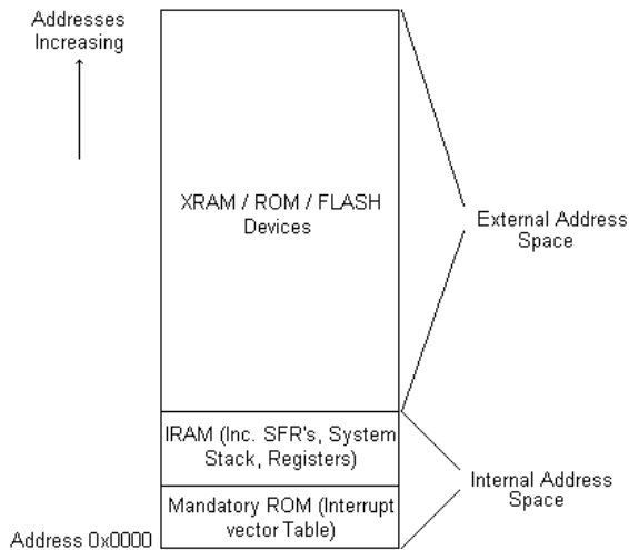
Fig. 3: Typical address space usage
