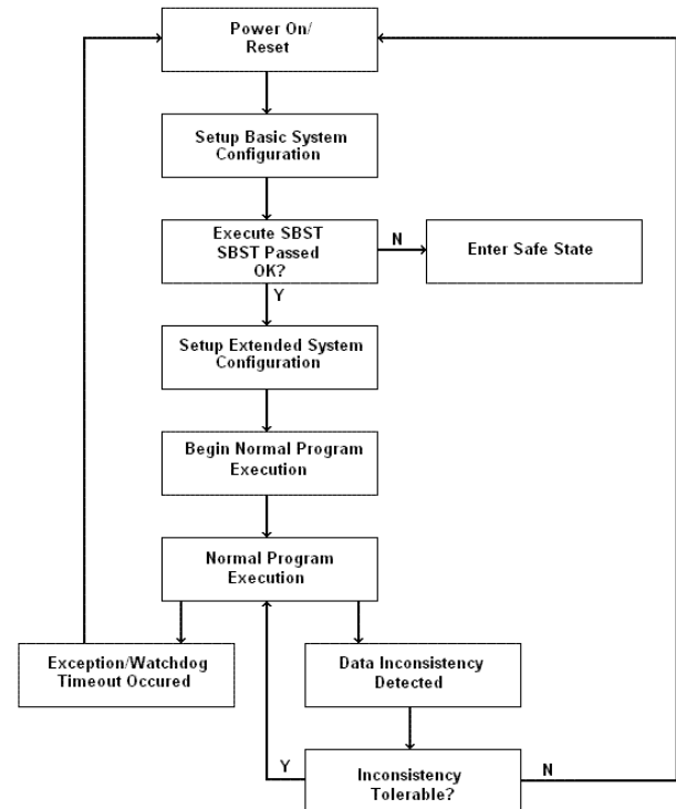
Fig. 7: Proposed approach to fault tolerance
