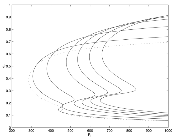
FIG. 4. Neutral-stability curves in the (\alpha_r, R_L) -plane for T_s = 0 (dotted line), 0.05, 0.15, 0.25, 0.30, 0.35 , and 0.40 (left to right).
