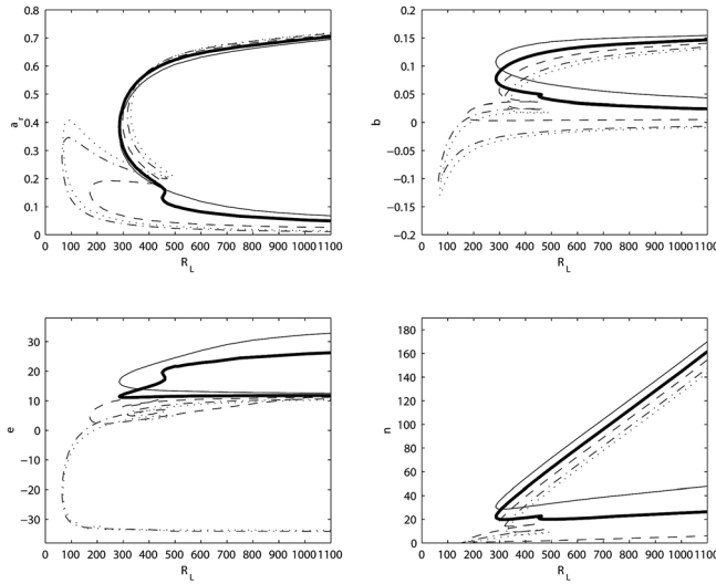
FIG. 9. Neutral-stability curves calculated in the rotating frame for \omega = 0 “—”; \omega = 4 “- -”; \omega = 7.9 “...”; \omega = 10 “- · - ·” ( T_s = 0 ).
