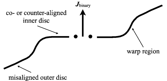
Figure 1. The warped disc shape expected after the inner disc co- or counteraligns with the binary plane but the outer disc stays misaligned. Eventually the entire disc will co- or counteralign with the binary plane, depending on the global criterion (equation 12). Note that in practice precession makes the warp non-axisymmetric.
