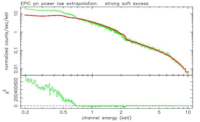
Fig. 5. Extrapolation of the power-law component down to soft X-ray energies. A strong soft excess component is detected below about 0.7 keV
