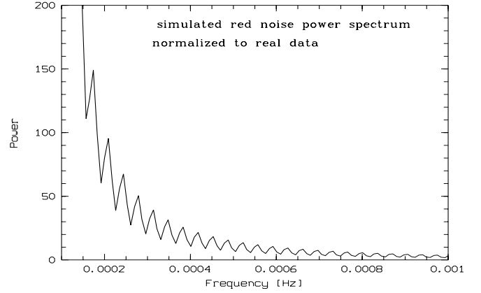
Fig. 4. Simulated red noise power spectrum of Mrk 766, normalized to the real data set
