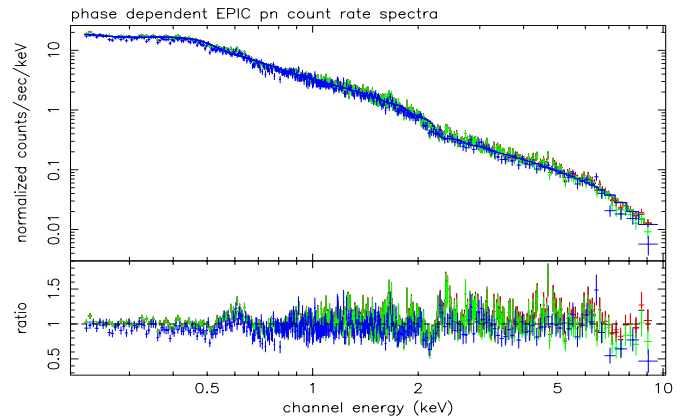
Fig. 6. Black body plus power-law fit to EPIC pn spectra selected from four different phase intervals. No significant changes in the black body temperature and the absorption by neutral hydrogen is detected
