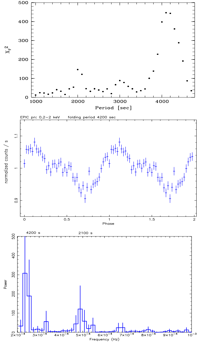
Fig. 2. Upper panel: reduced \chi^2_r versus the folding period for the 0.2–10 keV energy range. Middle panel: folded 0.2–2 keV light curve with the best fitting period of 4200 s. Lower panel: power spectrum for Mrk 766 in the 0.2–10 keV energy band
