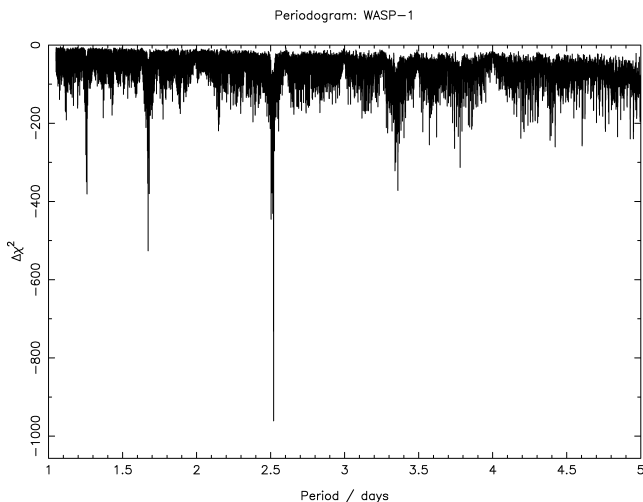
Figure 3. Periodogram output of HUNT1STAR for the unadulterated SuperWASP light curve of WASP-1. This is typical of the periodogram indicating the presence of a transiting planet, in this case WASP-1 b, which orbits with a period of about 2.52 d.
