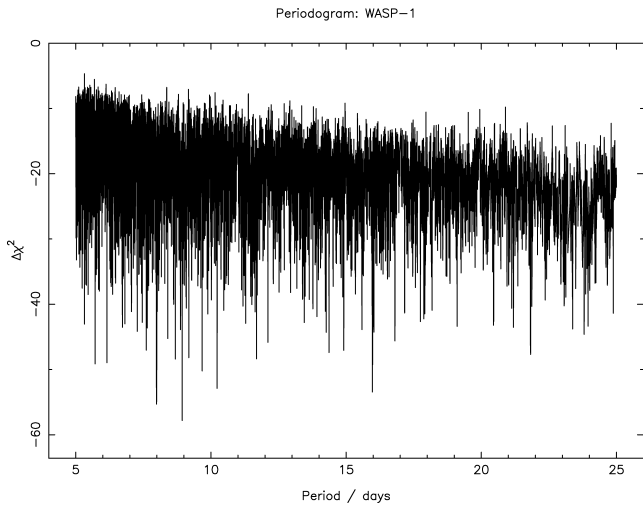
Figure 2. Periodogram output of HUNT1STAR for the residual light curve of WASP-1, after the subtraction of transits due to WASP-1 b. This is typical of the periodograms which exhibit no strong peaks.
