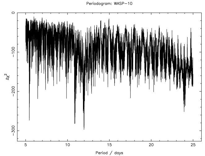
Figure 4. Periodogram output of HUNT1STAR for WASP-10. The strong peak observed at about 12 d is caused by stellar rotation with that period.
