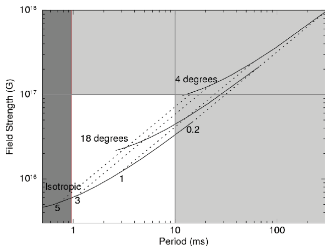
Figure 7. We show here the effect of beaming the emission of GRB 090515 assuming a mass of 1.4 M_{\odot} . Solid lines show isotropic solution and the solutions for the two beaming angles considered in Lyons et al. (2010). The dotted lines represent contours of equal redshift decreasing from left to right. The forbidden regions are as defined for Fig. 6(a).
