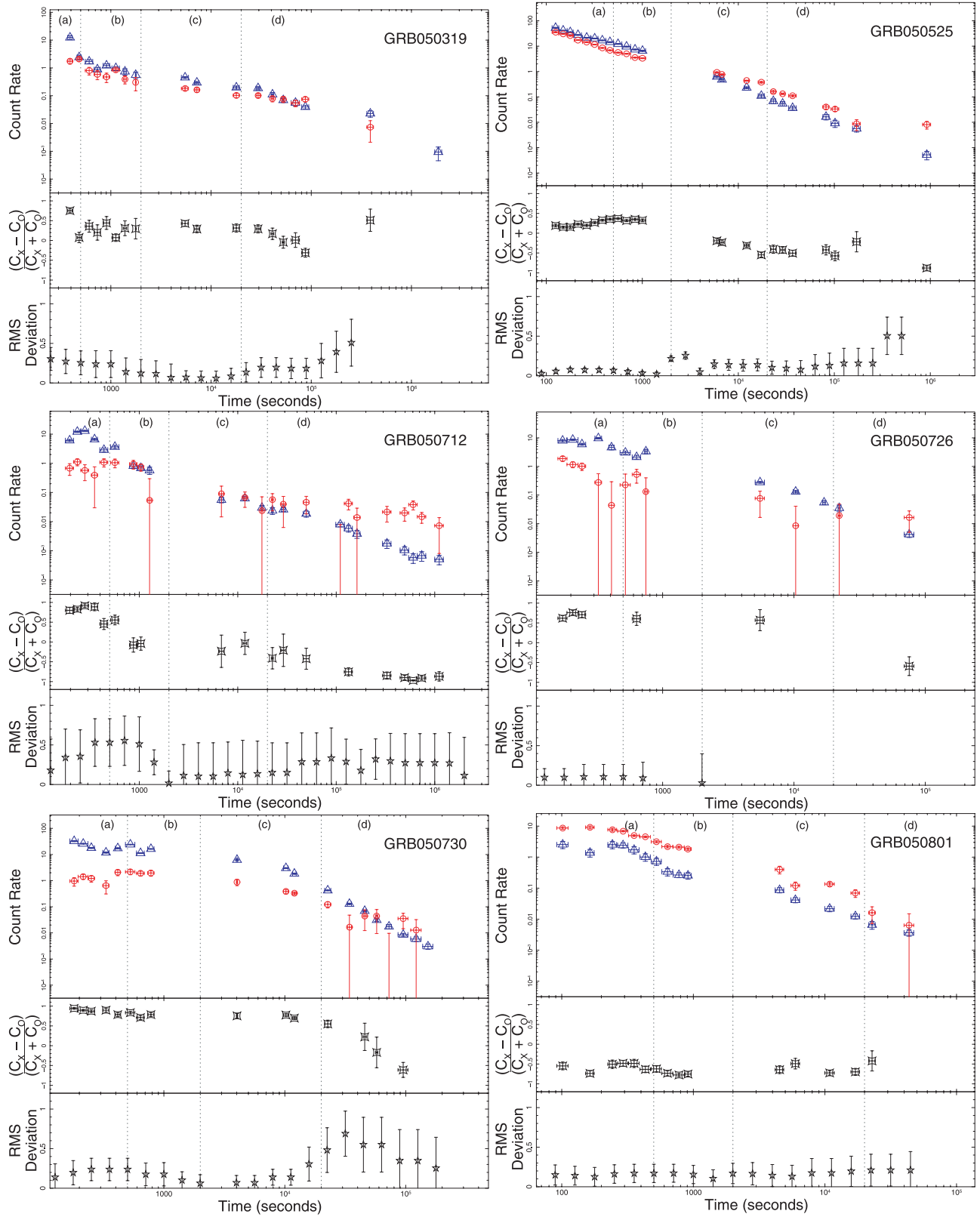
Figure 1. The 26 GRB X-ray and optical/UV afterglows. The dotted lines divide the light curves into the epochs (a)–(d), which are <500, 500–2000, 2000–20 000 and >20 000 s, respectively. The top pane of each panel shows the X-ray and optical/UV (equivalent to v -band) light curves. The X-ray light curves (blue triangles) have been binned to have the same bin sizes as the optical/UV data (red circles). The middle pane of each panel shows the X-ray to optical/UV hardness ratio, given by hardness ratio = (C_X - C_O)/(C_O + C_X) , where C_O is the v -band count rate and C_X is the X-ray count rate. The bottom pane of each panel shows the rms deviation of the logarithmic X-ray light curves relative to the logarithmic, normalized optical/UV light curves in a time window 1-dex wide. The window was shifted in steps of 0.15 in log time and the rms deviation was calculated for each window.
