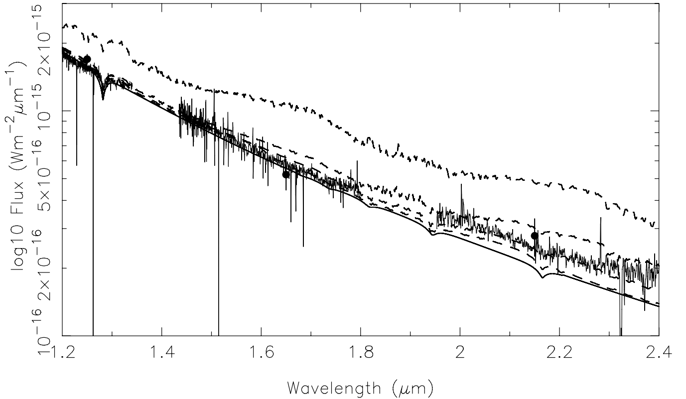
Figure 1. The GNIRS spectrum of WD 0137-349 from 1.2–2.4 \mu\text{m} compared to a synthetic white dwarf spectrum from a pure-H model atmosphere normalized using the observed V-band magnitude (solid line). Also shown is the synthetic white dwarf spectrum combined with spectra of known brown dwarfs scaled to the appropriate distance as follows (dashed lines, top-to-bottom): L0, L6, L8 and T5. Note the telluric water bands between 1.35–1.42 \mu\text{m} and 1.8–1.95 \mu\text{m} have been omitted.
