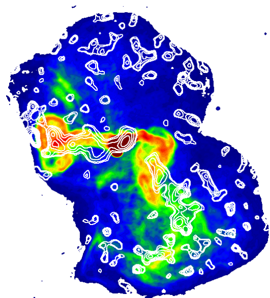
Fig. 8. The radio map at 90 cm, kindly provided by F. Owen, is shown with superimposed contours of MOS1 energy map. The contours are at [1000, 1002, 1004, 1006, 1008, 1010, 1011] mean energy level and the image as been smoothed with a Gaussian of \sigma = 40''
