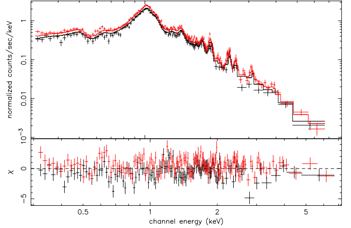
Fig. 5. MOS1 (black) and MOS2 (red) east arm spectrum and folded 2T model
