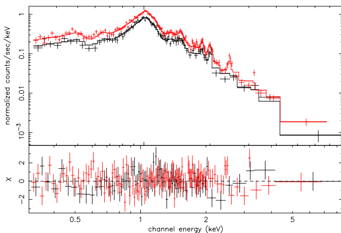
Fig. 6. M1 (black) & M2 (red) south-west arm spectrum and folded 2T model
