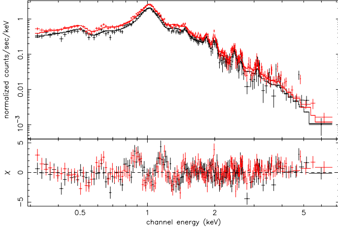
Fig. 4. The MOS E-arm spectrum and folded 1T model. Significant residuals are present at the energy of the FeL blend
