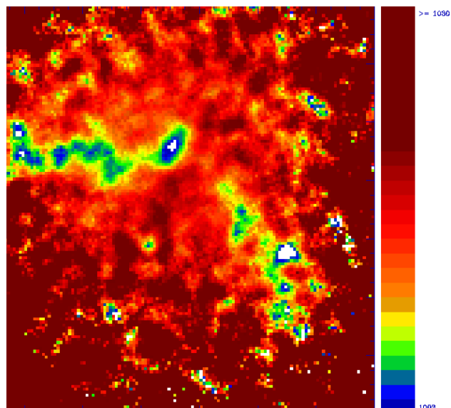
Fig. 3. MOS1 0.9–1.1 keV energy map (average of the energy of all photons falling in the same pixel). The image, smoothed by a Gaussian of \sigma = 12'' , is zoomed on the regions of interest (11 arcmin field of view). The color scale is in eV
