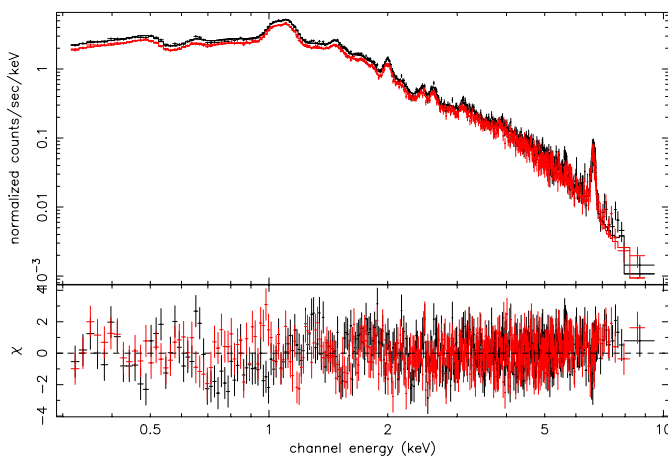
Fig. 7. M1 (black) and M2 (red) ambient medium spectrum and folded 1T model
