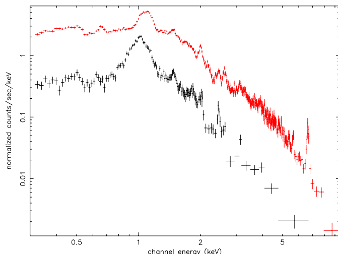
Fig. 2. MOS1 (in black) east arm spectrum compared with the surrounding ambient spectrum (in red)
