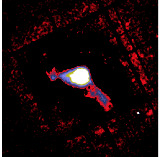
Fig. 1. Combined MOS1 and MOS2 0.2–10 keV image of the asymmetric extended X-ray arms; north is up, east is to the left. A model of the M 87 extended halo, obtained using the wavelet analysis, has been subtracted. The image covers a field of view of 17 arcmin
