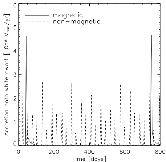
Figure 6. A plot showing accretion on to the WD as a function of time in magnetic and non-magnetic cases on the same time-scale as in Fig. 5. The magnetic outbursts have a higher peak accretion rate than the standard outbursts.
