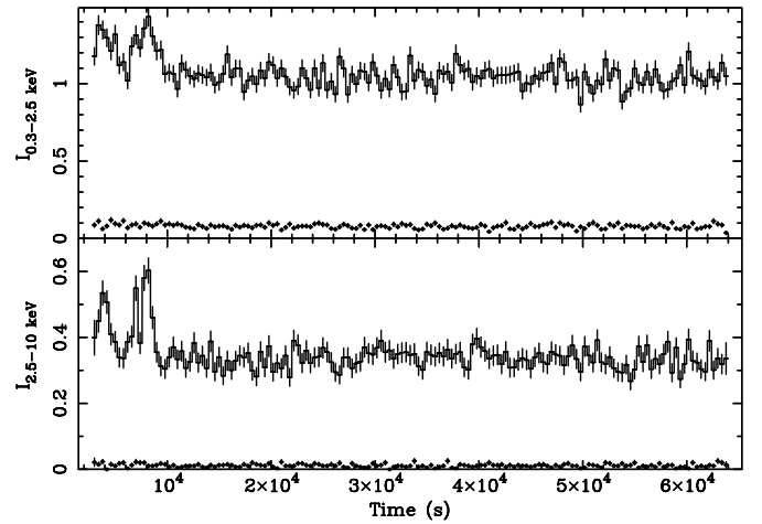
Fig. 2. The EPIC (PN + MOS1 + MOS2) lightcurves of RXJ0042.6+4115 from observation 4 in the 0.3–2.5 keV (top panel) and 2.5–10 keV (bottom panel) energy bands; the upper curve in each panel is the background-subtracted source curve, while the lower curve is the background curve. The lightcurves were accumulated with time bins of 400 s. Clearly, the amplitude of flaring is higher in the 2.5–10 keV energy band, and it is also clear that the background makes no contribution to the flares.
