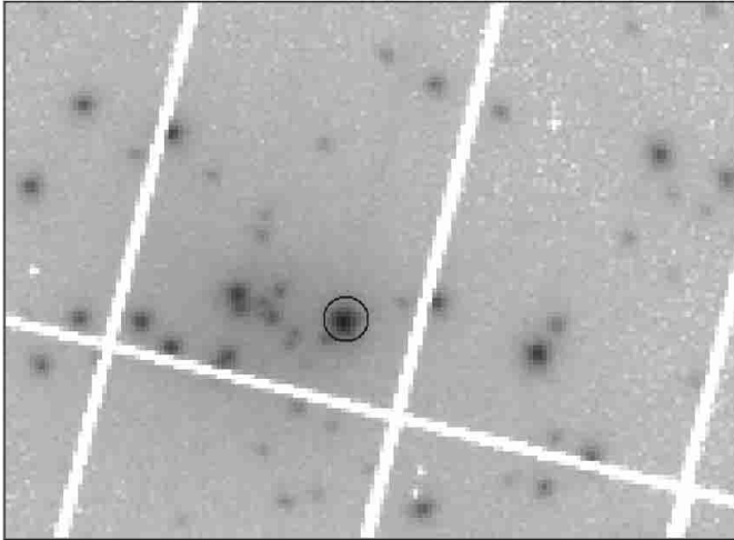
Fig. 1. A detail of the 0.3–10 keV PN image from the June 2001 XMM-Newton observation of the core of M31; north is up, east is left. The image is log scaled and 5' across. RXJ0042.6+4115 is circled in black, the circle defining the source extraction region.
