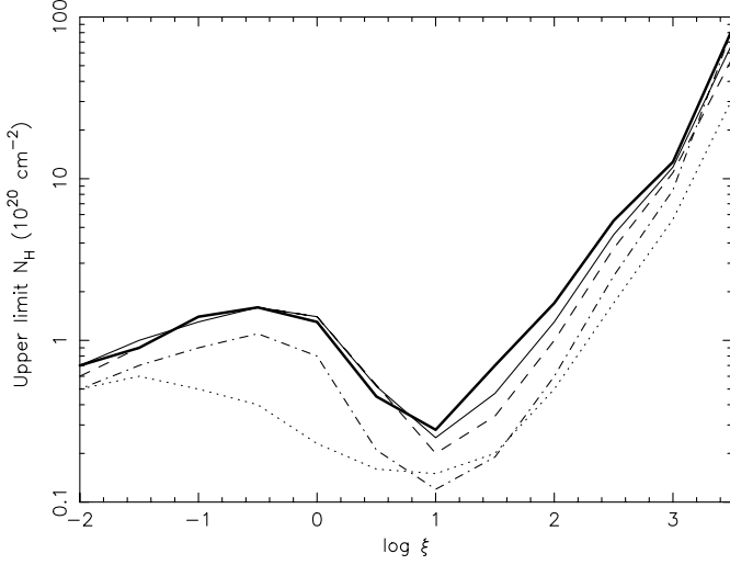
Fig. 5. Upper limit at 1\sigma of the column density N_H (expressed in 10^{20} \text{ cm}^{-2} ), versus the ionization parameter \xi (in logarithm scale). The curves correspond to different values of outflow velocities. Thick solid line: v = 0 \text{ km s}^{-1} , thin solid line: v = -250 \text{ km s}^{-1} , dashed line: v = -500 \text{ km s}^{-1} , dash-dot line: v = -1000 \text{ km s}^{-1} , and dots: v = -2000 \text{ km s}^{-1} .
