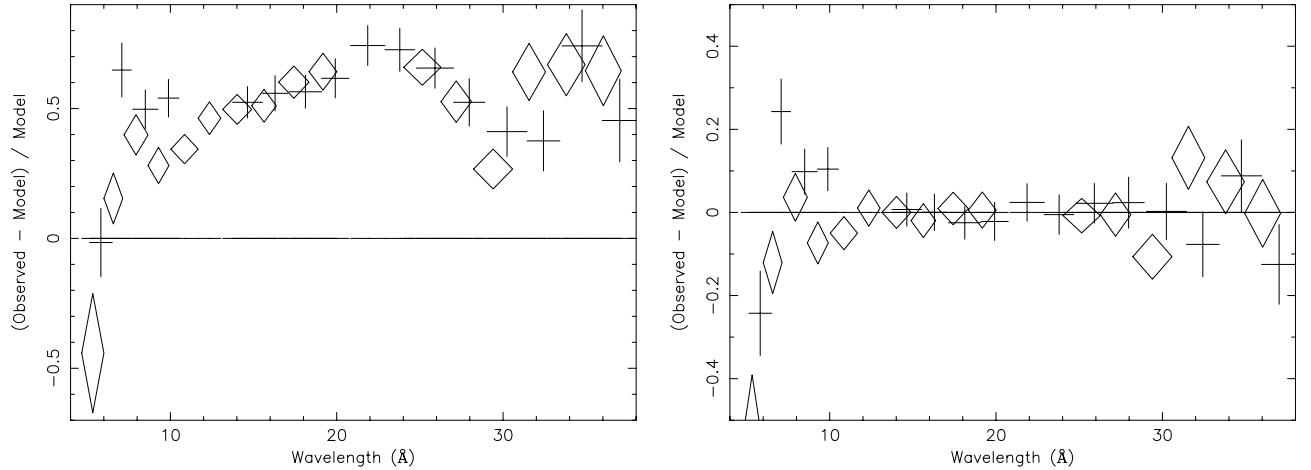
Fig. 4. The RGS fit residual spectra of ESO 198-G24 (observer frame) for the power-law (PL) model with the parameter fixed to the values found with EPIC. Left panel: PL only. Right panel: PL + “knak” model (see text for explanations). Crosses: RGS 1, diamonds: RGS 2.
