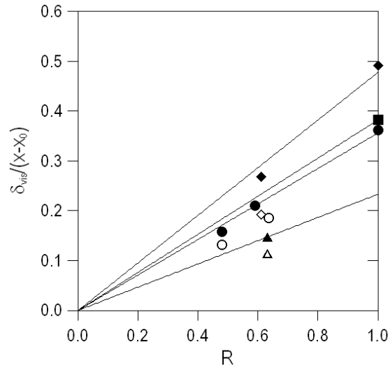
FIGURE 12. Visual-thickness growth rate vs. non-dimensionalised velocity difference between free streams: \rho_2/\rho_1=1.0 (circles), 2.0 (square), 7.2 (diamonds), 0.14 (triangles). Filled and unfilled symbols indicate organised and disorganised flow respectively. The reference lines are least-squares fits to the datum points for organised flow.
