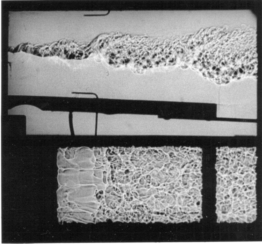
FIGURE 5. Simultaneous side- and plan-view spark shadowgraph showing mixing transition; U_1=13.1 m/s (helium), U_2=3.0 m/s (air).
