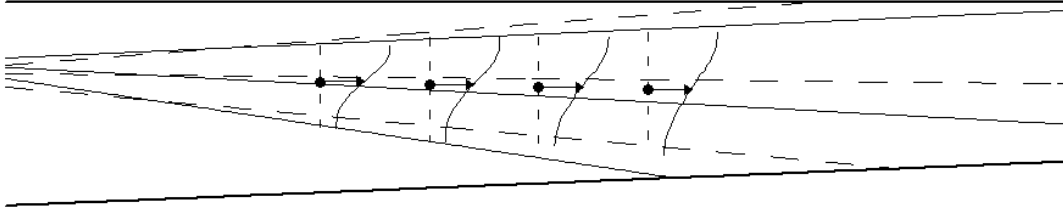
FIGURE 13. Orientations of self-similar mixing layer in its organised (continuous lines) and disorganised (broken lines) states for U_1=31.8 m/s, U_2=7.3 m/s, \rho_2/\rho_1=1.0 with walls of test section (bold lines) for reference. Also shown are four velocity profiles, the vector drawn on each profile indicating the transverse location at which the mean velocity was equal to the average of the free-stream values.
