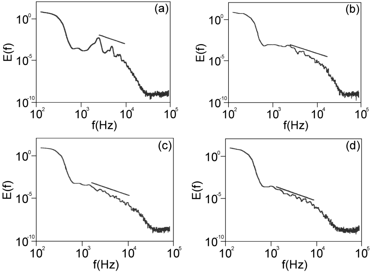
FIGURE 4. Power spectrum of velocity fluctuations at centre of mixing layer at distances of (a) 5 mm, (b) 15 mm, (c) 75 mm, (d) 110 mm from splitter plate; U_1=20.7 m/s, U_2=5.4 m/s, \rho_2/\rho_1=1.0 . Reference line indicates roll-off rate of fully developed inertial cascade.
