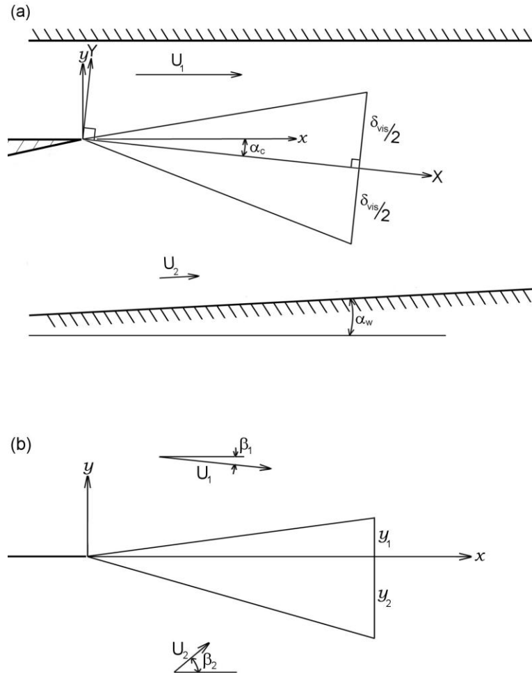
FIGURE 14. (a) Coordinate system for analysis of entrainment by experimental mixing layer. (b) Coordinate system for mixing-layer analysis of Abramovich.
