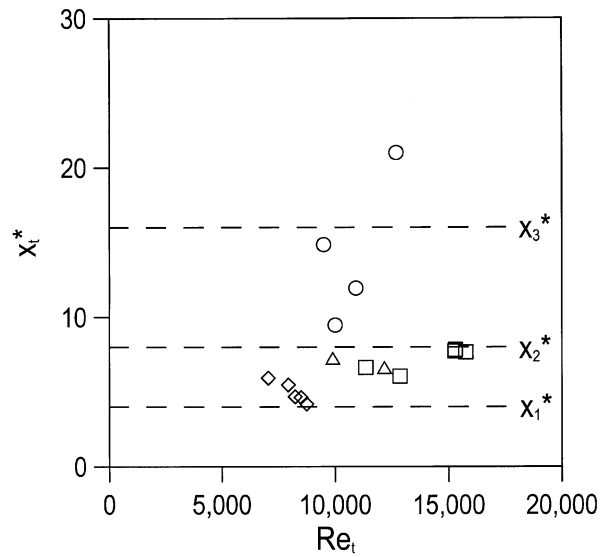
FIGURE 6. Mean transition location vs. transition Reynolds number: \rho_2/\rho_1=1.0 (circles and squares), 7.2 (diamonds), 0.14 (triangles). Circles indicate measurements made with nozzle/test-section build 1; all other measurements made with nozzle/test-section build 2.
