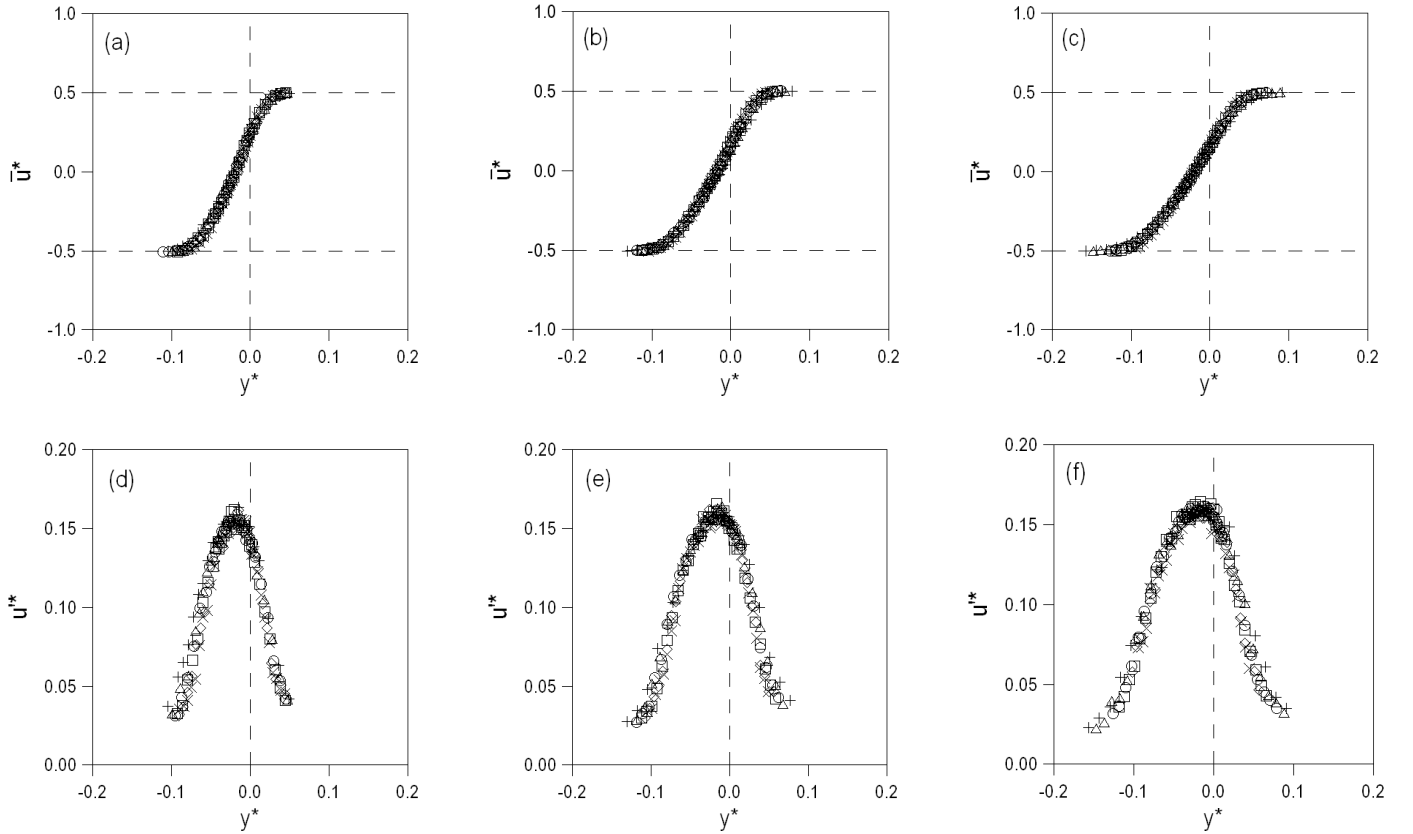
FIGURE 2. Non-dimensionalised profiles of (a)-(c) mean velocity and (d)-(f) root-mean-square of velocity fluctuations: (a) and (d) U_1=32.0 m/s, U_2=12.9 m/s; (b) and (e) U_1=32.1 m/s, U_2=9.6 m/s; (c) and (f) U_1=31.9 m/s, U_2=7.2 m/s; \rho_2/\rho_1=1.0 . Measurements made at distances of 72 mm (crosses), 97 mm (triangles), 122 mm (circles), 147 mm (squares), 172 mm (diamonds) and 197 mm (diagonal crosses) from splitter plate.
