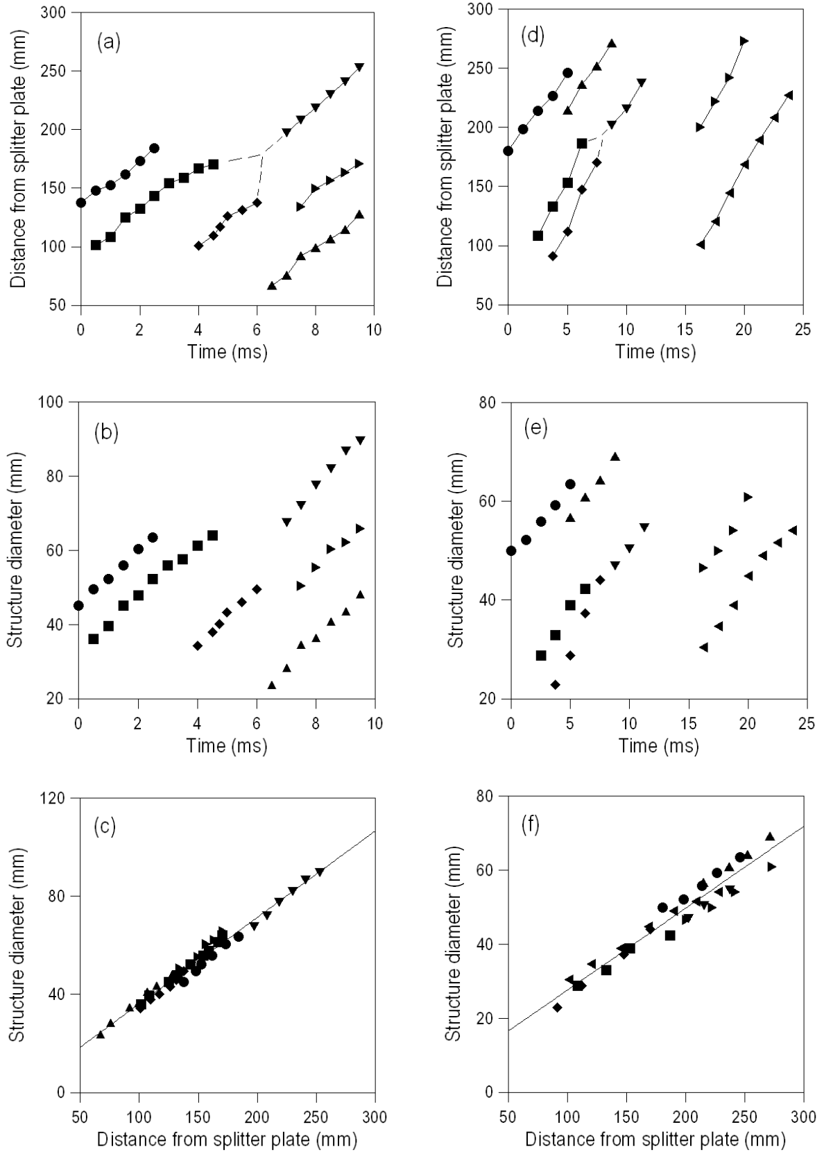
FIGURE 10. Post-transition large-structure evolution: (a)-(c) U_1=20.9 m/s, U_2=0 , \rho_2/\rho_1=1.0 ; (d)-(f) U_1=32.6 m/s, U_2=7.8 m/s, \rho_2/\rho_1=7.2 . Within each set of plots the same symbols are used to identify the individual structures.
