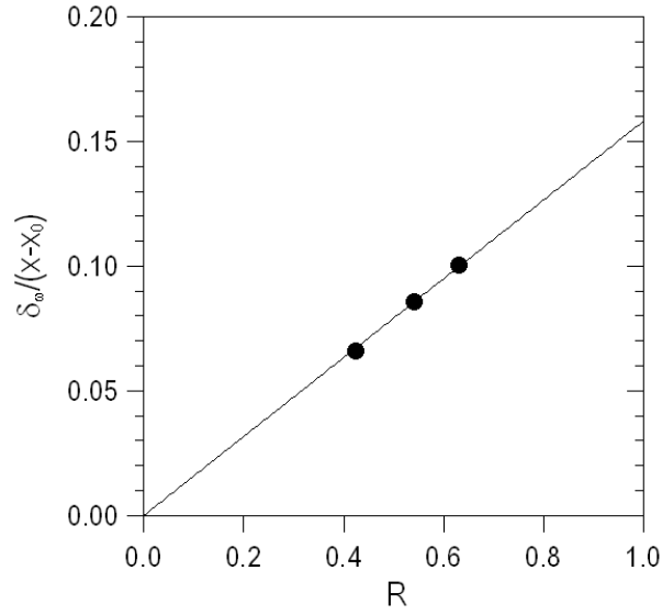
FIGURE 3. Vorticity-thickness growth rate vs. non-dimensionalised velocity difference between free streams; datum points computed from data presented in figure 2(a)-(c).
