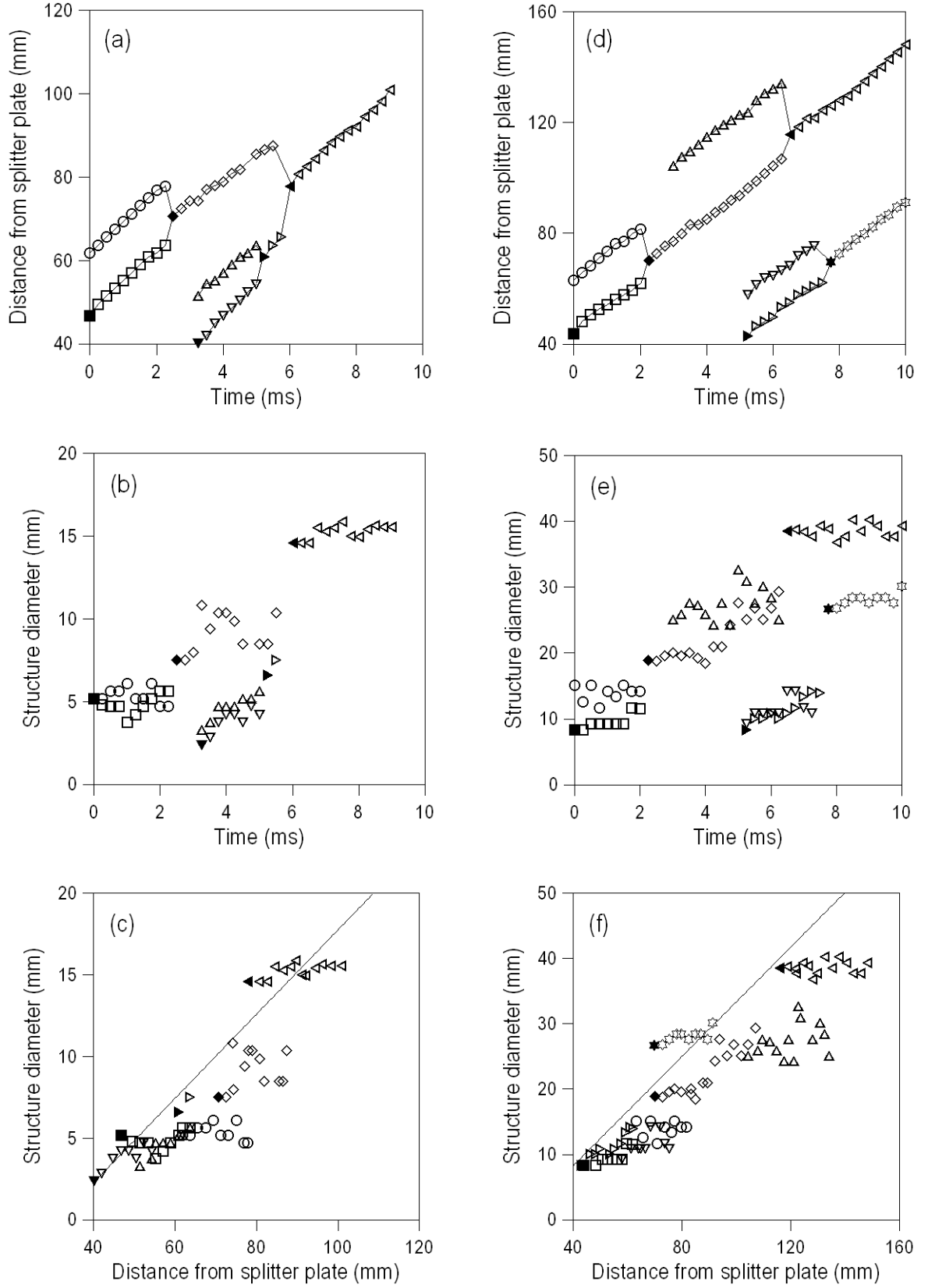
FIGURE 9. Pre-transition vortex evolution: (a)-(c) U_1=9.6 m/s, U_2=2.2 m/s, \rho_2/\rho_1=1.0 ; (d)-(f) U_1=18.1 m/s, U_2=4.3 m/s, \rho_2/\rho_1=7.2 . Within each set of plots the same symbols are used to identify the individual vortices. The reference lines in (c) and (f) are least-squares fits to the filled symbols only.
