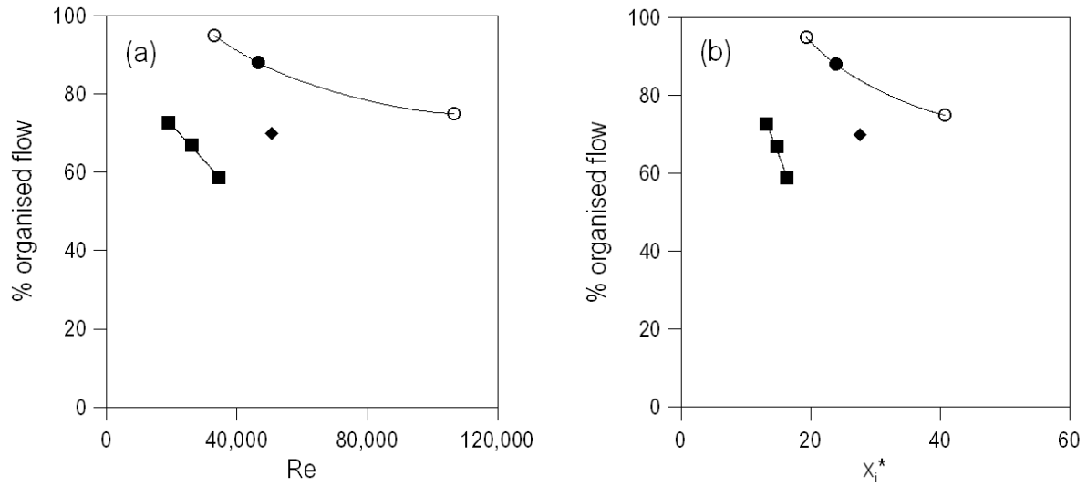
FIGURE 11. Extent of large-scale organisation in post-transition mixing layer (build 2 test section) vs. (a) Reynolds number and (b) pairing parameter at distance of 250 mm from splitter plate: \rho_2/\rho_1=1.0 (circles), 7.2 (squares), 0.14 (diamond). Filled symbols indicate test conditions for all of which R \sim 0.6 .
