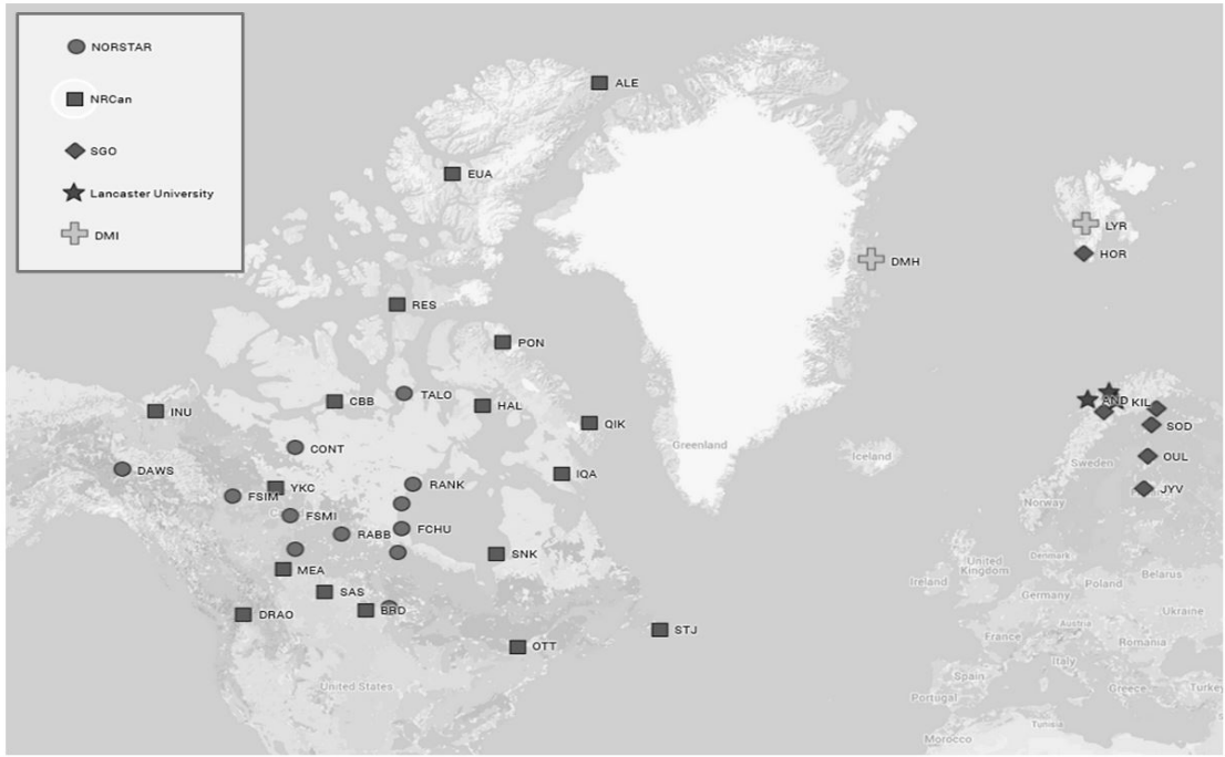
Figure 5. Selected riometers in the Global Riometer Array (GloRiA).
