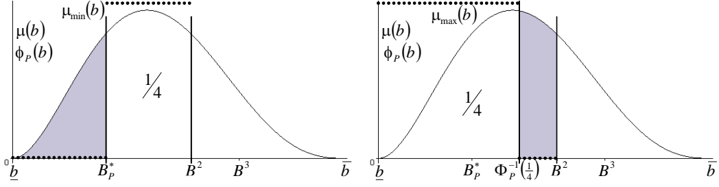
Figure A1: Households' allocation with randomisations \mu_{\min}(b) and \mu_{\max}(b) .
