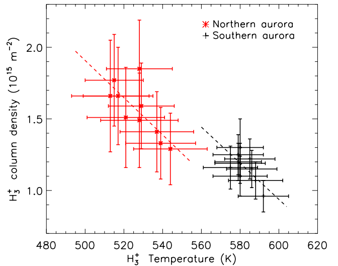
Figure 2. The \text{H}_3^+ temperature and density derived from Keck NIRSPEC observations of Saturn’s northern (stars) and southern (crosses) aurora from the 2013 April 17 (O’Donoghue et al. 2014). The Pearson correlation coefficient between temperature and density for the northern aurora is -0.72 and -0.52 for the south, making them high and moderately correlated, respectively. The dashed lines show the un-weighted linear fit to each hemisphere, clearly showing the anticorrelation.
