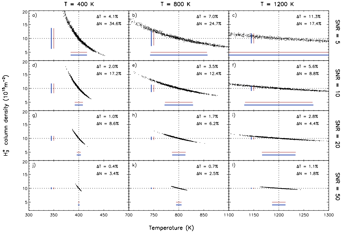
Figure 4. The fitted H_3^+ density as a function of temperature for fixed temperatures of 400, 800 and 1200 K, and for SNRs of 5, 10, 20 and 50. Each plot contains 1000 points, each signifying an individual fit to a synthetic H_3^+ spectrum at temperature T . The bold blue line shows the standard deviation in both temperature (horizontal) and density (vertical) of these fits, and the thin red line shows the average errors on these two parameters, as given by the fitting routine. These two lines are always similar within a few per cent. The percentage error on both parameters is also given. The higher the SNR, the better constrained the H_3^+ temperature and density becomes.
