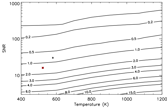
Figure 5. The percentage error of the \text{H}_3^+ temperature ( \Delta T/T ) as a function of SNR and fitted temperature. The black cross and the red star show the southern and northern aurora of Fig. 2, respectively.
