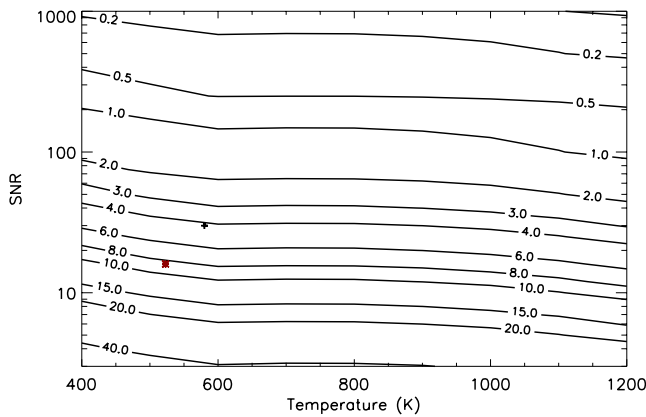
Figure 6. As Fig. 5 but showing the percentage error on the \text{H}_3^+ column density ( \Delta N/N ).
