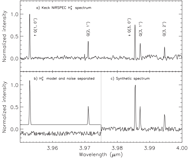
Figure 3. (a) The Keck NIRSPEC H_3^+ spectrum of Saturn's northern aurora, covering 14 min of exposure (7 min on Saturn). The H_3^+ line assignments are indicated, all of which are from the Q -branch ( \Delta J = 0 ). This spectrum fits to T = 528 \pm 17 K and N = 1.8 \pm 0.3 \times 10^{15} \text{ m}^{-2} . (b) The H_3^+ spectral model (offset by +0.1 in y ), and the random noise (offset by -0.1 in y ). (c) The two model components combined, comparing well to the actual NIRSPEC observations of (a).
