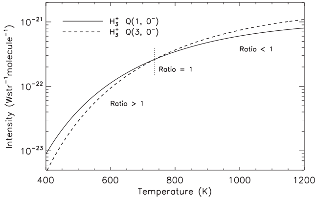
Figure 1. The intensity of the \text{H}_3^+ Q(1, 0^-) at 3.953 \mu\text{m} (solid) and \text{H}_3^+ Q(3, 0^-) at 3.986 \mu\text{m} (dashed) lines as a function of temperature. The two lines evolve at different rates, and the ratio of the two can be used a proxy for the temperature. The dotted line indicates where the ratio of the two lines is equal to 1, occurring at a temperature of 737 K.
