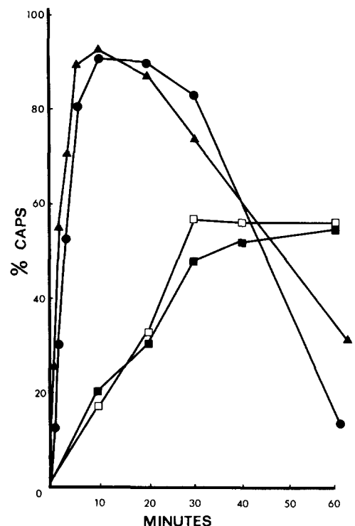
FIGURE 4 Kinetics of capping of surface Ig and cholera toxin bound to mouse lymphocytes. All ligands were bound at 0°C, and the temperature raised to 37°C for the times indicated. After fixing, the number of cells displaying a cap was counted. The results are expressed as a percentage of the ligand-positive cells. ●, FITC-labeled goat anti-mouse Ig (1:40 dilution). ▲, Rabbit anti-mouse Ig (1:30) followed by FITC-labeled goat anti-rabbit Ig (1:50). □, Cholera toxin (100 ng/ml) followed by horse anti-toxin (1:10) and FITC-labeled swine anti-horse Ig (1:50). ■, Cholera toxin B subunit (100 ng/ml) followed by horse anti-toxin (1:10) and FITC-labeled swine anti-horse Ig (1:50).
