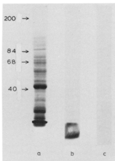
FIGURE 1 Identification of cholera toxin binding molecules in mouse lymphocytes. Total cellular proteins (150 µg/track) were resolved in 7.5% SDS polyacrylamide gels, and the cholera toxin binding components identified by overlaying gel tracks with ^{125}\text{I} -labeled toxin ( 3 \times 10^6 cpm in 0.75 ml of PBS/0.1% BSA specific activity 22 µCi/µg) in conjunction with autoradiography, as described in Materials and Methods. (a) Coomassie Blue-stained total cell protein. (b) Track overlaid with ^{125}\text{I} -labeled cholera toxin. (c) As in Fig. 2 b, except the ^{125}\text{I} -labeled cholera toxin was preincubated with 50 µg/ml of bovine brain mixed gangliosides (Sigma Chemical Co., Poole, Dorset, England) for 1 h at 0°C.
