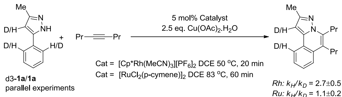
Scheme 5 Parallel KIE experiments
