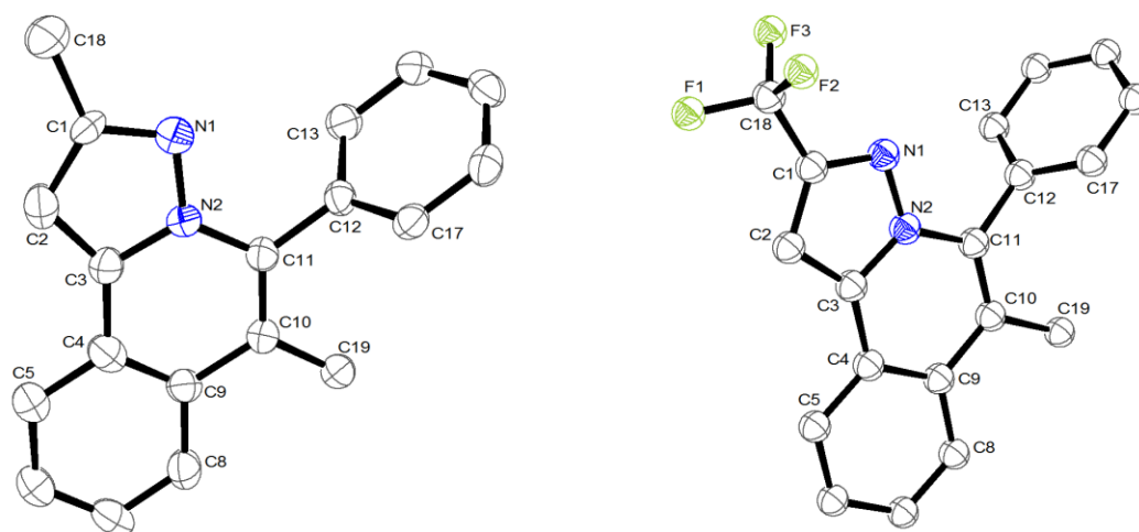
Figure 1. Ortep plots of 3ac (left) and 3dc (right). Thermal ellipsoids are drawn at 50% probability and hydrogen atoms are omitted for clarity.
