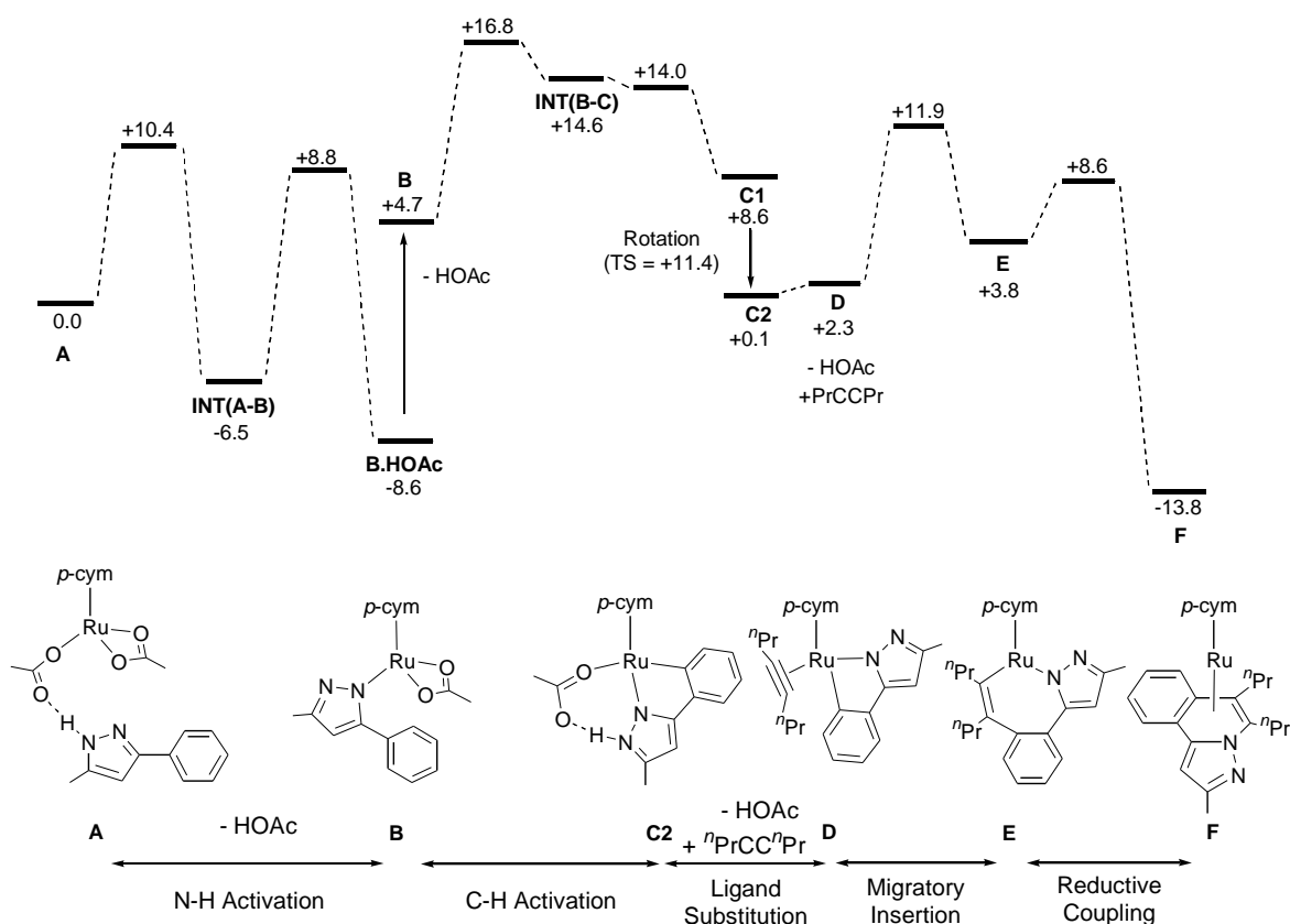
Figure 7: Computed reaction profiles ( G_{MeOH} , kcal/mol) for the coupling of {}^n\text{PrCC}^n\text{Pr} with 1a at \text{Ru}(\text{OAc})_2(p\text{-cymene}) (BP86-D3 protocol)
