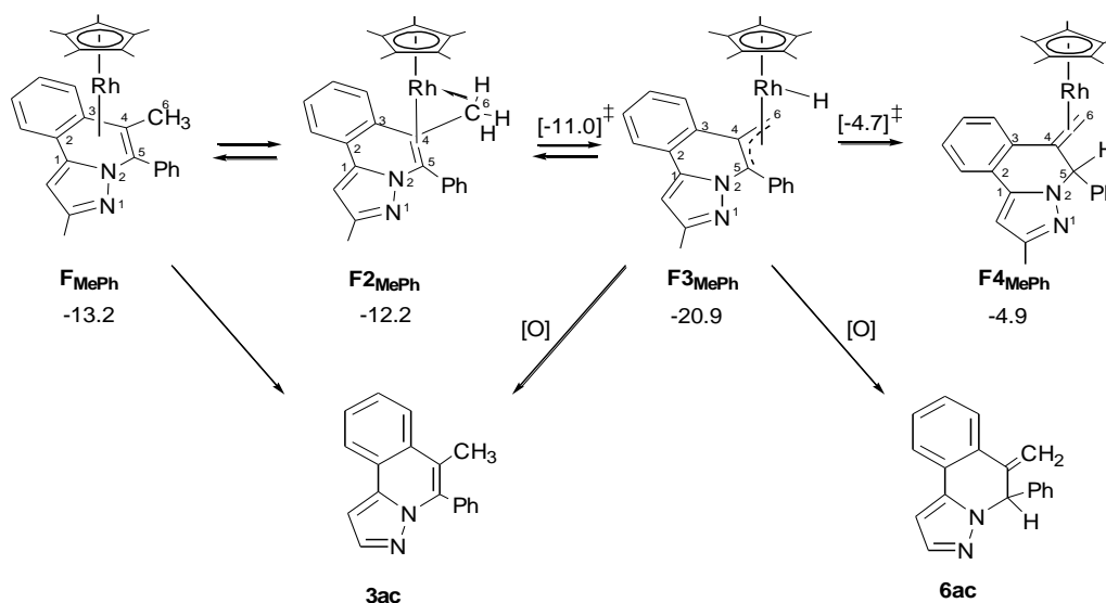
Figure 6. Possible mechanism of formation of isomerised heterocyclic product 6ac . Relative free energies ( G_{\text{DCE}} , kcal/mol) are computed with the BP86-D3 protocol.
