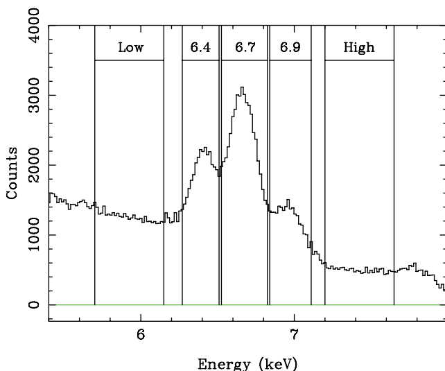
Figure 1. The full-field spectrum from the pn camera (Obs ID: 0202670801) in the region of the Fe-K lines. The underlying continuum was sampled in two narrow bands (marked ‘Low’ and ‘High’) at energies immediately below and above the Fe-K complex. The various narrow bands are delineated by the vertical lines.
