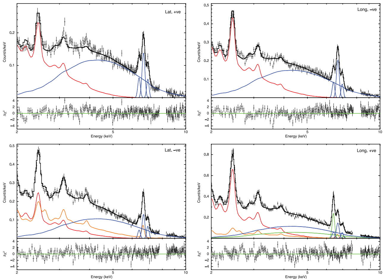
Figure 6. X-ray spectra measured by the pn camera in observation 020670801 in four regions: upper-left panel: the Lat +ve region; upper-right panel: the Long -ve region; lower-left panel: the Lat -ve region; lower-right panel: the Long +ve region. Each panel shows the X-ray spectrum after background subtraction in the 2–10 keV band, excluding the region around the Cu K\alpha instrumental line. The best-fitting model and the fitting residuals are also shown. The contribution of different spectral components is illustrated by the different colour curves – blue: the 7.5 keV thermal bremsstrahlung continuum plus iron lines associated with unresolved sources; green: the fluorescent iron line and reflected continuum from dense molecular clouds; red: soft thermal emission with kT = 0.8 keV; orange: (relatively) soft thermal emission with kT = 1.5 keV.
