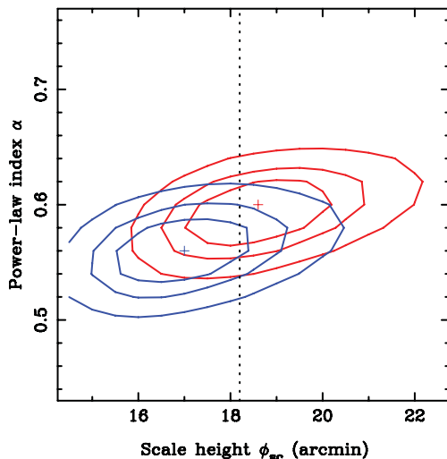
Figure 5. The variation of \chi^2 as a function of the source model parameters, \alpha and \phi_{sc} . The contours represent the 68, 90 and 99 per cent confidence intervals. The results from the pn data are shown in red and those from the combined-MOS data in blue. The dashed vertical line is drawn at 18.2 arcmin; this corresponds to the scale height of 45 pc reported for the NSD by Launhardt et al. (2002) (see text).
