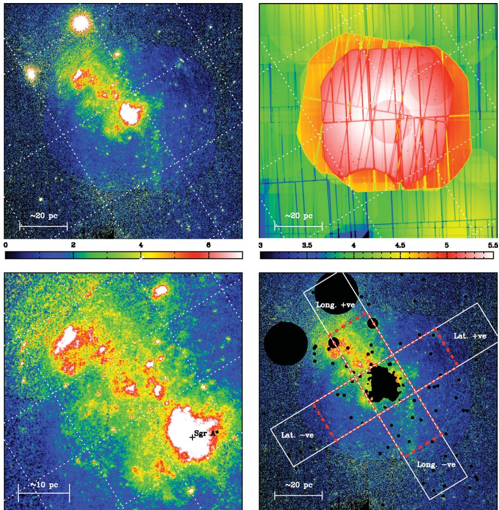
Figure 2. Image mosaics based on XMM–Newton observations covering a central 43.2 \times 43.2 arcmin 2 field ( 100 \times 100 pc at the GC). The images are constructed on a celestial coordinate grid with east to the left. Upper-left panel: 2–10 keV pn image. The adjacent colour bar is calibrated in units of pn counts per pixel per 20 ks. Upper-right panel: the corresponding pn exposure map. The adjacent colour bar is calibrated in units of \log_{10} of the exposure (s). Lower-left panel: a blow-up of the 2–10 keV image showing the region to the north-east of Sgr A*. Lower-right panel: the 2–10 keV pn image overlaid by a spatial mask which removes the most luminous sources (see Section 2.2). The longitudinal and latitudinal spatial cuts are represented by the two intersecting white rectangles, which have long-axis dimensions of \pm 22 arcmin and full widths of 8 arcmin (see Section 2.3). The red boxes (of dimension 8 \times 9 arcmin 2 ) define the four regions from which spectral data were extracted (see Section 2.4). In three of the panels the white dotted lines represent a Galactic coordinate grid with a 15 arcmin spacing.
