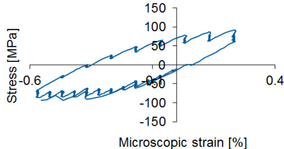
Fig. 4 Macroscopic stress-strain responses for // Mg AZ31at 150^\circ\text{C}
