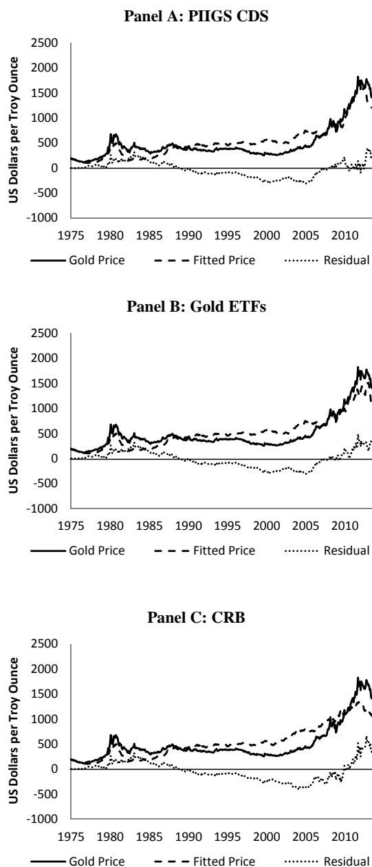
Figure 5: Alternative Proxies
