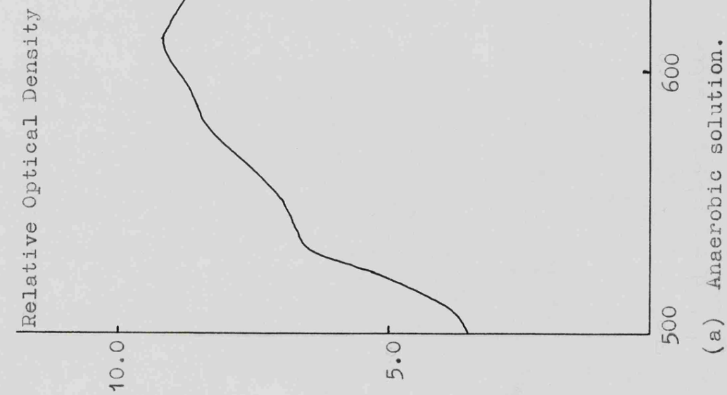
Figure 10. Spectra of transient species obtained by flash photolysis of acetonitrile solutions of tri-p-tolylamine. ( t = 25\mu s )
