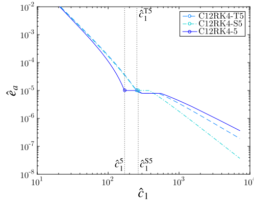
Fig. 7. Comparison of the error estimated by Eq. (24) among the C12RK4-5, C12RK4-T5 and C12RK4-S5 schemes. Symbols indicate (\hat{k}^*, \hat{\sigma}^*) values.
