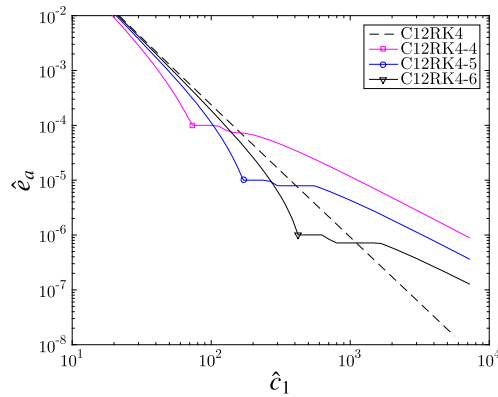
Fig. 6. Error estimated by Eq. (24) as a function of \hat{c}_1 for C12RK4- n schemes, one-dimensional implementation. Symbols indicate (\hat{k}^*, \hat{\sigma}^*) values.
