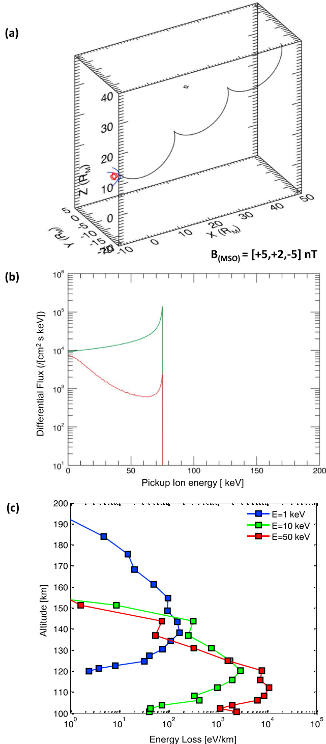
Figure 5. (a) Birth point of pickup ions reaching the sampling location for simulation case 7 (Table 1). Mars is in red, the bow shock in blue, and Siding Spring is a black diamond. (b) Omnidirectional differential flux of pickup O^+ versus energy for Mars hot oxygen exosphere (red) and comet Siding Spring (green) for case 7. (c) Simulation of the energy loss for 1-, 10-, and 50-keV O^+ test particles launched radially toward Mars at 300 km. MSO = Mars-Solar-Orbital.
