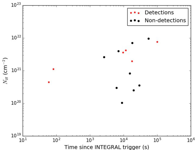
Figure 4. Plot of T_{\text{START}} against Galactic N_H of all of our 15 WEAK triggers including both XRT detections and non-detections.
