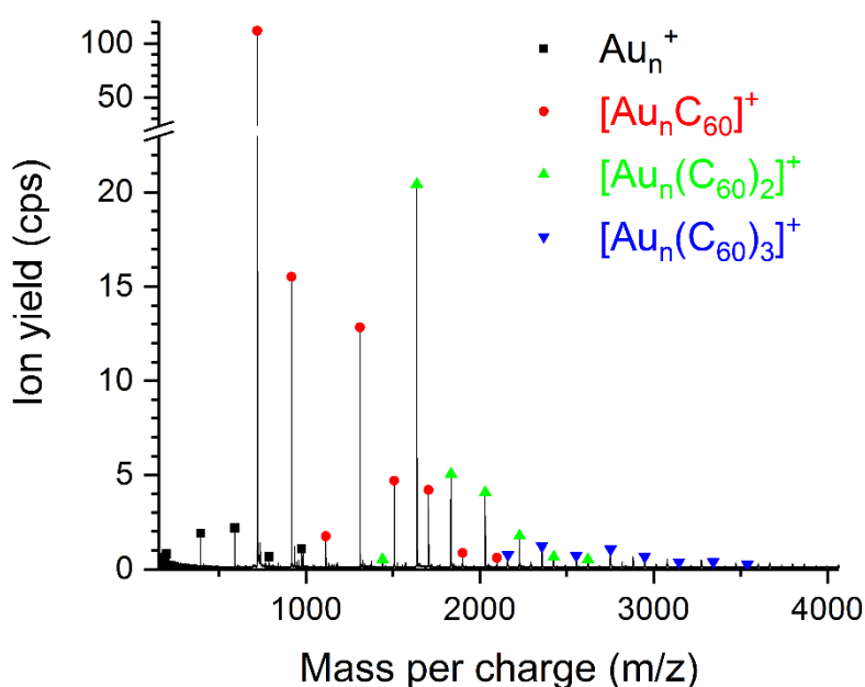
Figure 2. Mass spectrum of [\text{Au}_n(\text{C}_{60})_m]^+ cations. For the series of peaks identified as coming from [\text{Au}_n\text{C}_{60}]^+ , [\text{Au}_n(\text{C}_{60})_2]^+ and [\text{Au}_n(\text{C}_{60})_3]^+ , note that each series begins at n = 1 .
