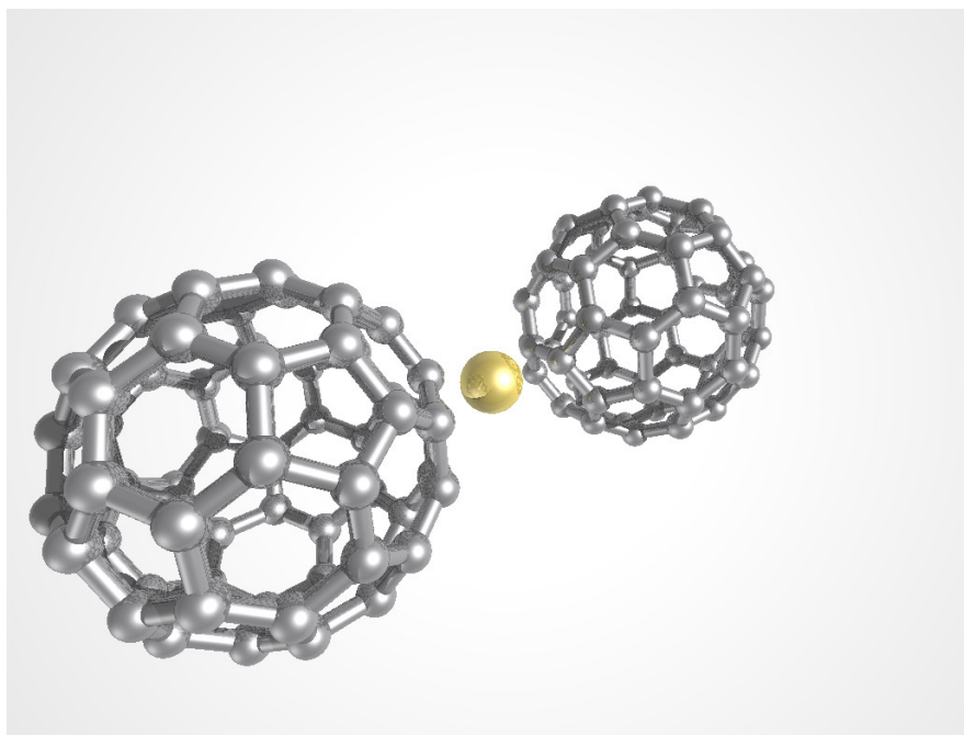
Figure 3. Calculated lowest energy structure of [\text{Au}(\text{C}_{60})_2]^+ .
