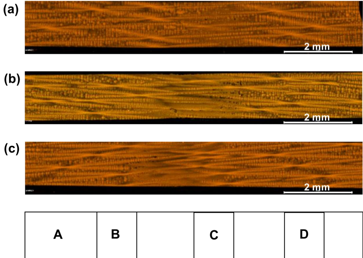
Fig. 11: Re map using Micro X-ray fluorescence along the gauge length in the as-cast cooling experiments; (a) sample \mathbf{U}_1 , (b) sample \mathbf{M}_3 , (c) sample \mathbf{L}_2 .
