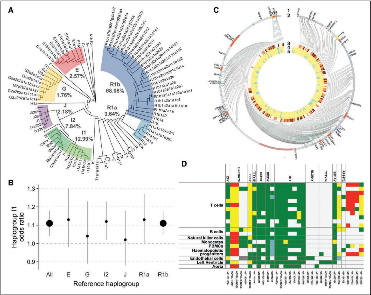
Figure 1. The Y chromosome and coronary artery disease. A , Phylogenetic analysis of the Y chromosome in UK Biobank. Colored (matched to Hallast et al) groups of tree branches examined for association with coronary artery disease (CAD) and their respective frequencies. B , Odds ratios for CAD in men with haplogroup I1 compared with men with other haplogroups of the Y chromosome. Error bars show the lower and upper bounds of the 95% CI. The size of the point reflects the level of statistical significance after correction for multiple testing (associations that survived the correction for multiple testing are shown as large points). C , Two hundred thirty-five genetic variants specific to haplogroup I1 uncovered through DNA sequencing of male-specific region of the Y chromosome (MSY). Variant locations are visualized as radial lines (2) originating in the outermost gray circle in the context of known protein-coding genes (red boxes), noncoding genes (yellow), and pseudogenes (blue boxes) of the Y chromosome; gene symbols are external to the outermost circle (1). Links to the inner circles are colored in green for variants mapping to genes and gray for intergenic variants. The number of datasets in which each variant appears (3) is scaled from light yellow (1) to dark red (3). Single-nucleotide substitutions are shown in yellow and insertion-deletions in turquoise (4). Novel variants are also highlighted in turquoise (5). D , Thirty-one genetic variants exclusive to haplogroup I1 shown in context of the summarized Roadmap Epigenomics chromatin states from 21 epigenomes of relevance to atherosclerosis/CAD. Individual epigenomes are grouped under the same type of cell/tissue. Red denotes a transcription start site state; yellow, an enhancer state; green, a transcribed state; and pale gray, a silent state. MSY gene symbols are annotated above the heat map variant identifier (wherever present).
