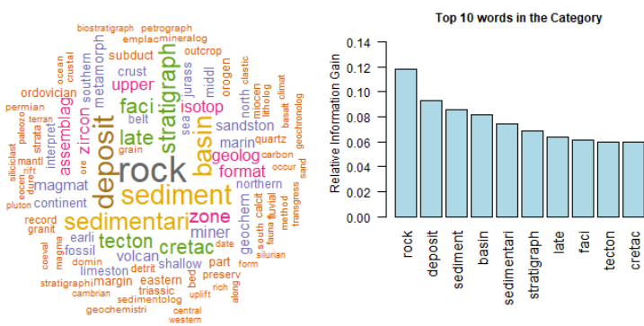
FIGURE 198. Geology
