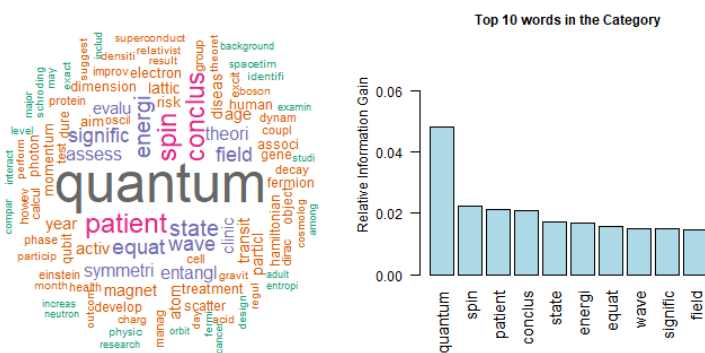
FIGURE 32. Physics, Multidisciplinary
