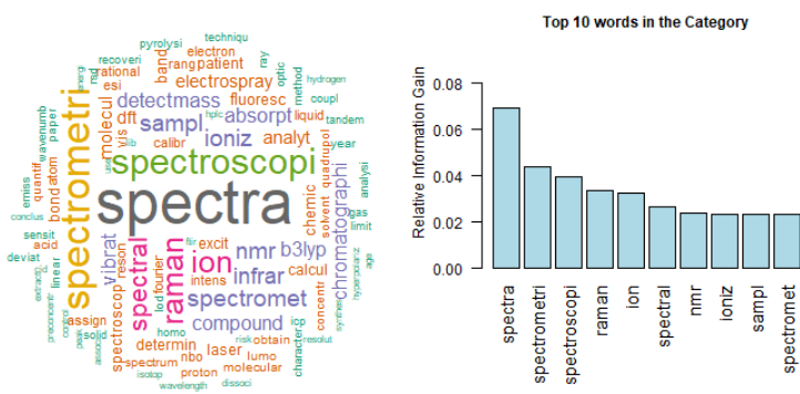
FIGURE 116. Spectroscopy
