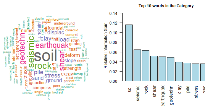
FIGURE 149. Engineering, Geological
