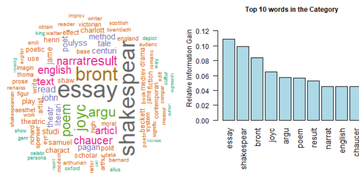
FIGURE 247. Literature, American
