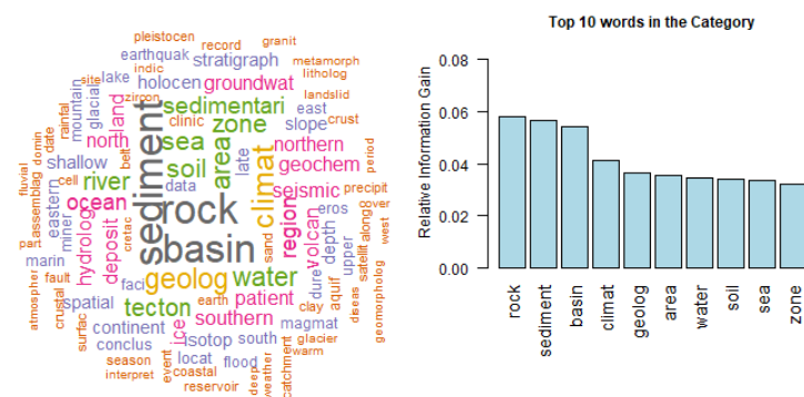
FIGURE 30. Geosciences, Multidisciplinary
