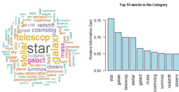
FIGURE 33. Astronomy & Astrophysics
