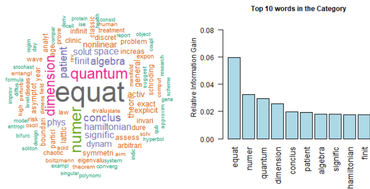
FIGURE 84. Physics, Mathematical
