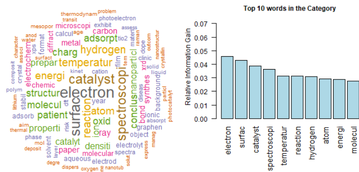
FIGURE 4. Chemistry, Physical
