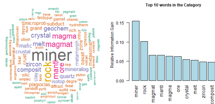
FIGURE 187. Mineralogy
