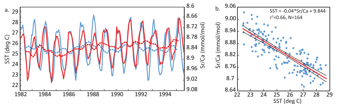
Figure 5. Calibration of monthly coral Sr/Ca. (a) Time series of monthly OI SST (blue lines; grid centered at 55°E, 21°S; Reynolds et al., 2002) and monthly coral Sr/Ca data measured at La Reunion (red lines) for the time period 1982–1995. Thick dashed lines are 13-point moving averages of monthly data. (b) Linear OLS regression of monthly coral Sr/Ca versus OI SST with 95% confidence levels. See text for discussion.
