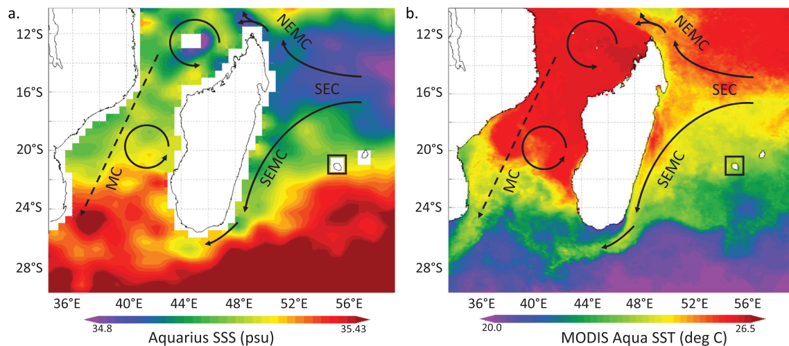
Figure 1. Monthly SSS and SST in the SW Indian Ocean. (a) Map of mean monthly SSS (Aquarius OISST, 1^\circ \times 1^\circ grid) and (b) mean monthly SST (MODIS Aqua daytime SST, 4 km resolution) during August 2013 in the SW Indian Ocean. The SEC can be seen as a low-salinity, warm water current that bifurcates at the coast of Madagascar. The location of La Reunion is indicated by a black rectangle. Charts computed with Live Access Server LAS8.6 ( http://apdr.csoest.hawaii.edu , date of access 26 March 2019).
