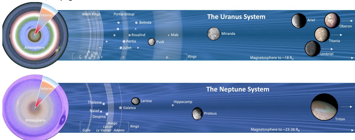
Fig. 1. The Uranus and Neptune systems, from false-colour representations of the atmosphere (southern poles) and interior, to the ring and satellite systems. The position of rings and satellites in the inner systems are to scale with the planetary radii, but the relative sizes of the satellite images are not. Arrows next to major moons indicating that they orbit at larger planetocentric distances. The magnetosphere and radiation belts would encompass the full area of the figure. Credit: L.N. Fletcher/M. Hedman/E. Karkoschka/Voyager-2.
