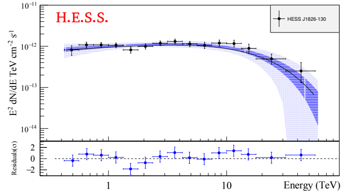
Fig. 3. VHE \gamma -ray spectrum of HESS J1826–130 extracted from the green circular source region shown in Fig. 1. The black dots show the flux points with 1\sigma statistical errors. The 1\sigma and 3\sigma error bands of the best-fit ECPL model are shown with the blue and light blue shaded regions, respectively, while the best-fit ECPL model itself is shown with the black line. The spectrum shown is binned such that all flux points have a minimum significance level of 2.0\sigma . The significance of the last flux bin centered at 42.7 TeV is 2.4\sigma .
