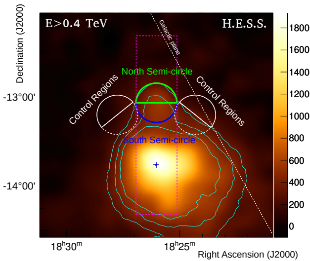
Fig. 4. VHE \gamma -ray excess map of HESS J1826–130 for all events saturated for a better visualization, showing the north semi-circle (green), south semi-circle (blue), and control regions for both north (solid white) and south (dashed white) semi-circle regions. The control regions are distributed in a radially symmetric manner around the peak position of HESS J1825–137, indicated with the blue cross, obtained from the dataset and for energies above 0.4 TeV. The cyan contours indicate the significance of the emission at the 15\sigma , 20\sigma and 25\sigma levels.
