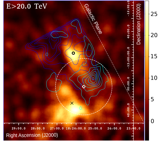
Fig. 5. VHE \gamma -ray excess map of HESS J1826–130 for events above 20 TeV, together with total column density map contours. The black circle and cross show the location of the pulsars PSR J1826–1256 and PSR J1826–1334. The cyan and blue contours show the total column density contours of [2.5, 9.5] \times 10^{22} \text{ cm}^2 , derived from Nobeyama ^{12}\text{CO}(1-0) and SGPS HI data, for gas velocities between 45–60 \text{km s}^{-1} (d: 4 kpc) and 60–80 \text{km s}^{-1} (d: 4.6 kpc), respectively. The white dashed circle and diamond are the extension and best-fit position of recently reported E > 100 TeV emitting source, eHWC J1825–134 (HAWC Collaboration 2020).
