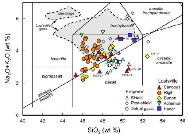
Fig. 4. A plot of total alkalis against silica (after Le Bas et al. , 1986), showing the range of composition of volcanic rock samples with <2 wt% LOI recovered from the Louisville seamounts during IODP Expedition 330, and by dredging and drilling on the Emperor seamounts (from Regelous et al. , 2003; Huang et al. , 2005). All analyses have been recalculated to sum to 100 wt% with Fe as FeO. The line separating Hawaiian tholeiitic and alkaline basalts is from Macdonald & Katsura (1964). The field of analyses of Louisville glass samples (from Nichols et al. , 2014) covering the same drilled interval as the whole-rock samples is shown in grey. It should be noted that many of the least altered whole-rock samples appear to have lost alkalis.
