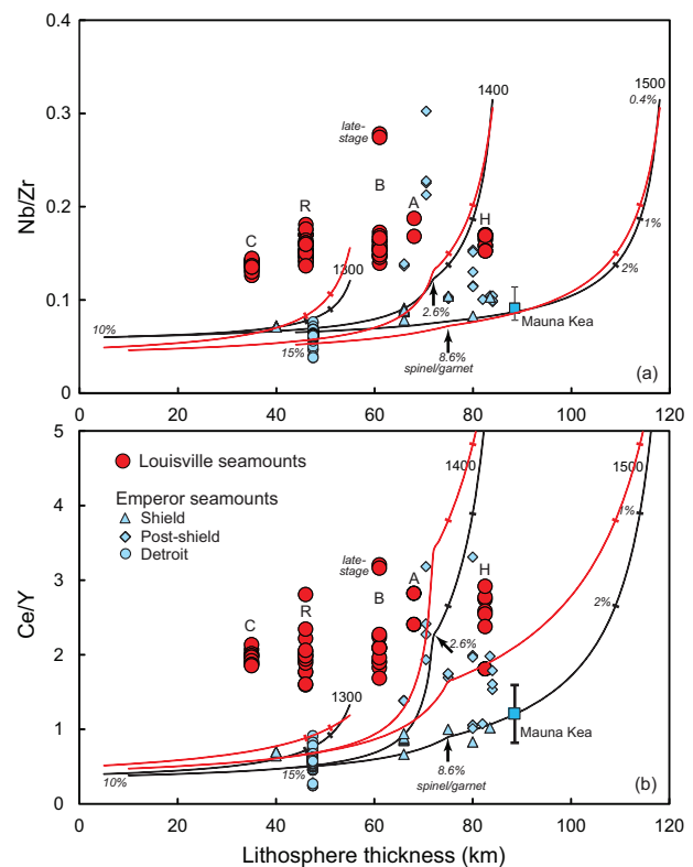
Fig. 10. Curves showing the variation of Nb/Zr and Ce/Y with lithosphere thickness in accumulated partial melts from mantle with T_p = 1300 , 1400 and 1500^\circ\text{C} , based on the melting model shown in Fig. 9. The black curves are for a peridotite mantle source; red curves are for a 50:50 mixture of peridotite and pyroxenite–eclogite. Nb/Zr and Ce/Y are calculated by summing the composition of partial melts in 1 km (0.4%) increments in a column of mantle extending from the depth of the dry solidus to the base of the lithosphere. The small arrows mark the points at which the curves cross the garnet–spinel transition, and the numbers give the melt per cent at various points along the curves. Lithosphere thickness for the data points is calculated from the age of the lithosphere at the time of eruption and the relationship between age and the depth to the 1100^\circ\text{C} isotherm in the plate model of McKenzie et al. (2005). Data from Detroit Seamount (Huang et al. , 2005) plot close to the curve for T_p = 1500^\circ\text{C} , and data from the post-shield stage plot between the curves for T_p = 1400^\circ\text{C} and 1300^\circ\text{C} . This is consistent with the derivation of shield-forming magmas from the hotter axis of a mantle plume and the post-shield magmas from the cooler plume sheath as the seamount drifts away from the plume axis. The mean composition (error bars show the full range of the data) of shield-forming lavas of Mauna Kea, sampled by the Hawaii Scientific Drilling Project (Rhodes & Vollinger, 2004), plots close to the curve for T_p = 1500^\circ\text{C} . Data from the Louisville seamounts, by contrast, show no significant relationship between Nb/Zr and Ce/Y and lithosphere thickness at the time of seamount formation. C, Canopus; R, Rigil; B, Burton; A, Achernar; H, Hadar.
