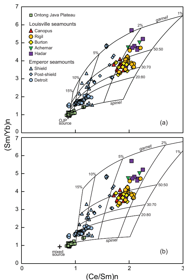
Fig. 7. Chondrite-normalized Sm/Yb plotted against chondrite-normalized Ce/Sm for basalt samples from the Emperor (data from Regelous et al. , 2003; Huang et al. , 2005) and Louisville seamounts. Data (from Fitton & Godard, 2004) for basalt from the Ontong Java Plateau (OJP) are included for comparison. (a) Partial melting curves are based on a mantle source composition derived from the composition of primitive OJP tholeiitic (Kroenke-type) basalt and are labelled with melt per cent and proportion of spinel- and garnet-lherzolite in the source. (b) The melting curves are for a mantle source composed of a 50:50 mixture of peridotite and pyroxenite-eclogite. Details of the melting calculations are given in the text, and the D values used are given in Table 4.
