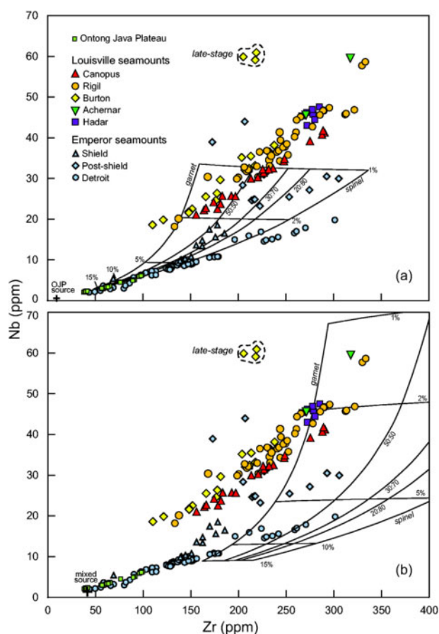
Fig. 8. Nb plotted against Zr for basalt samples from the Emperor (data from Regelous et al. , 2003 ; Huang et al. , 2005 ) and Louisville seamounts. Data for basalt from the Ontong Java Plateau (OJP) are included for comparison. (a) Partial melting curves are based on a peridotite mantle source composition derived from the composition of primitive OJP tholeiitic (Kroenke-type) basalt and are labelled with melt per cent and proportion of spinel- and garnet-lherzolite in the source. (b) The melting curves are for a mantle source composed of a 50:50 mixture of peridotite and pyroxenite-eclogite. Details of the melting calculations are given in the text, and the D values used are given in Table 4 . The late-stage samples from Burton seamount include two glass analyses from Nichols et al. (2014) .
