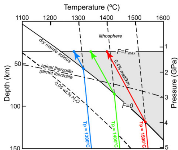
Fig. 9. A decompression melting model for mantle with potential temperature ( T_p ) of 1300, 1400 and 1500 °C. The mantle has an adiabatic gradient of 0.3 °C km -1 (Turcotte & Schubert, 1982) until it crosses the dry solidus and cools at a faster rate, producing melt at 0.4 % km -1 (Klein & Langmuir, 1987). Decompression and melting stop at the base of the lithosphere. The dry mantle solidus and the solidus of mantle with 0.05 wt.% water are from Katz et al. (2003), and the depth of the transition from spinel- to garnet-lherzolite is from Klemme & O'Neill (2000).
